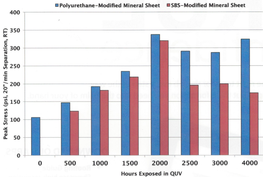
Figure 7 – ASTM D412 testing on UV-exposed cast films of polyurethane-modified bitumen vs. SBS-modified bitumen.
